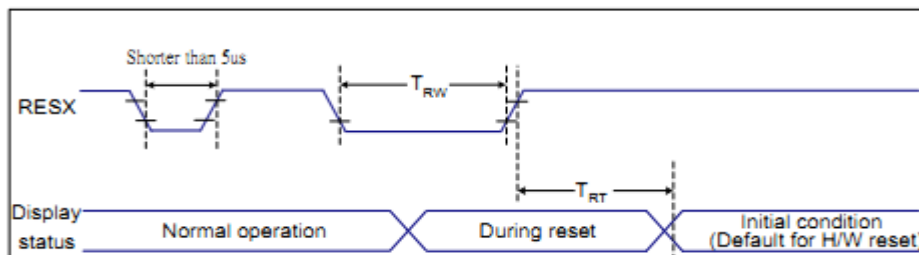
Figure 10 Reset Timing
