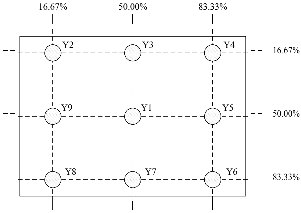
Fig.7-1 Measuring point
