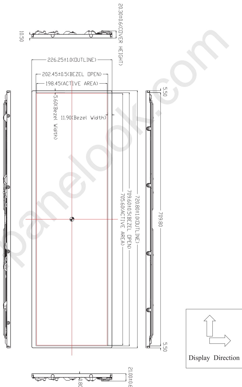
&lt; Figure 3.TFT-LCD Module Outline Dimensions (Front View) &gt;
