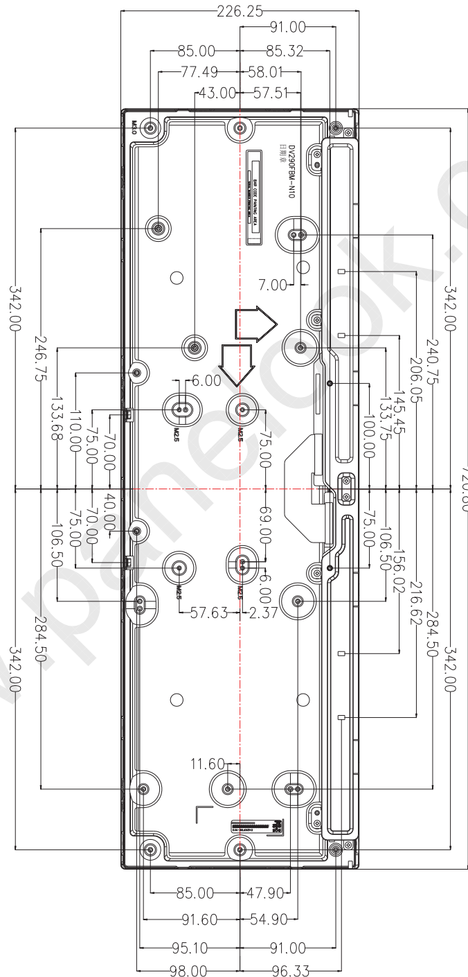
&lt; Figure 4.TFT-LCD Module Outline Dimensions (Rear View) &gt;
