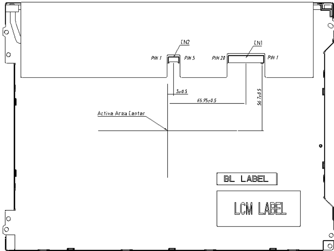
Figure 20 Reference Outline Drawing (Back Side)
