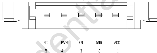
Figure 9 LED Connector
