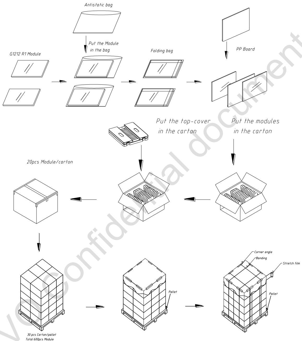
Figure 23 Packing Method
