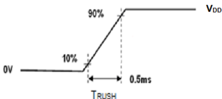
Figure 15 V_{DD} Rising Time
